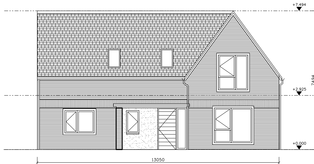
FRONT ELEVATION
