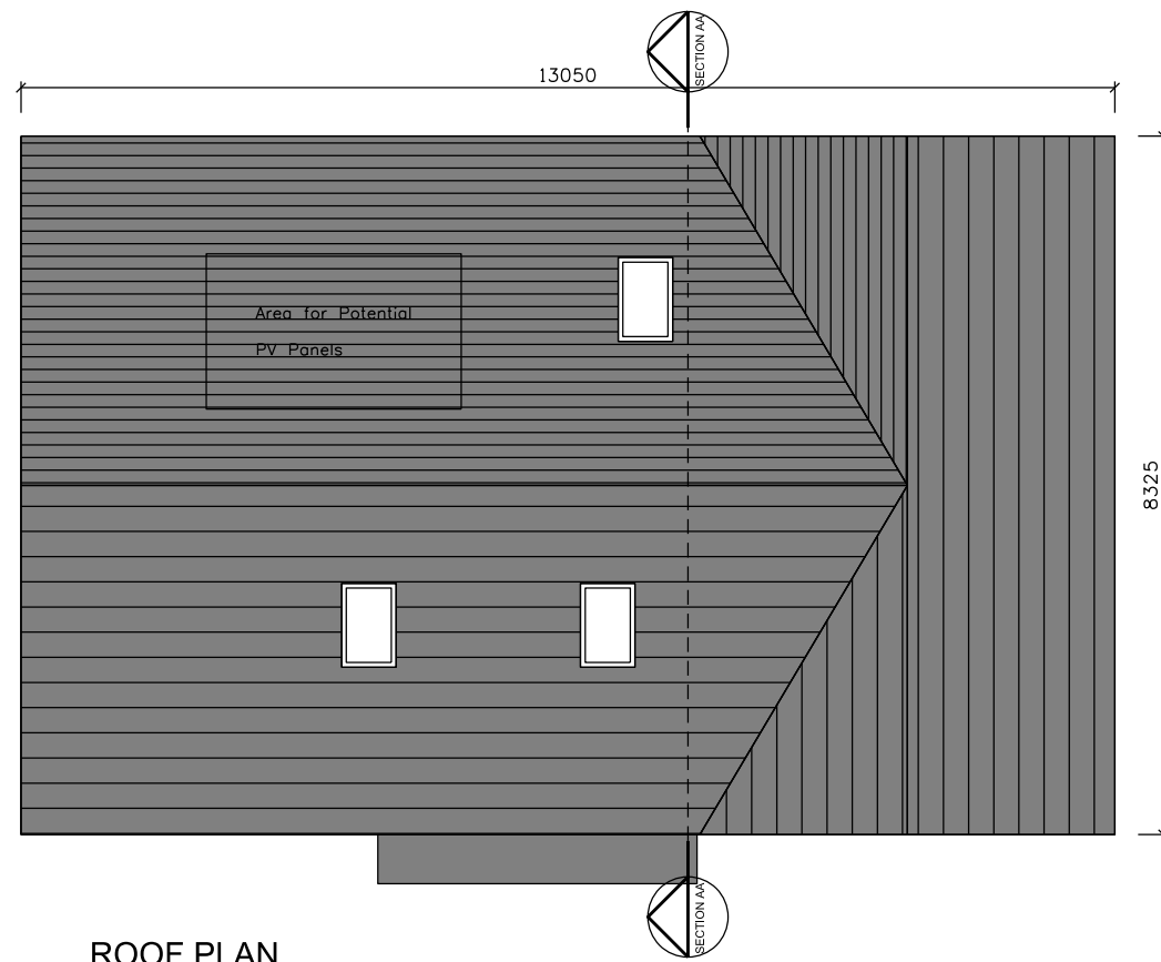
ROOF PLAN
